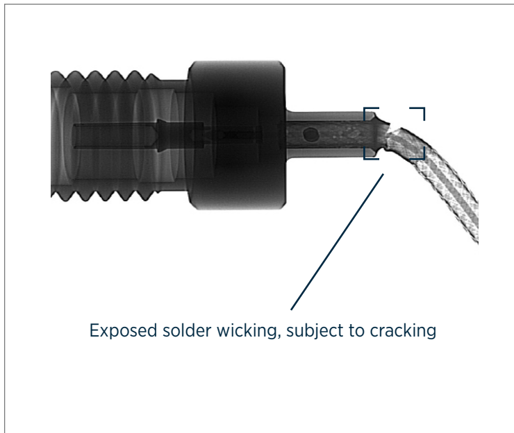
Figure 1: Cable assembly with damage caused by bending in the solder wicking area
